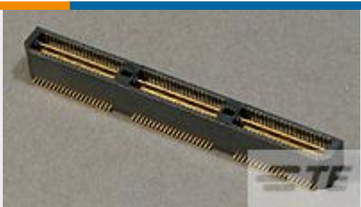
TE Part # 5-1658464-3 MSB0.80PL8ASY84DP,GP,30,VCTR
